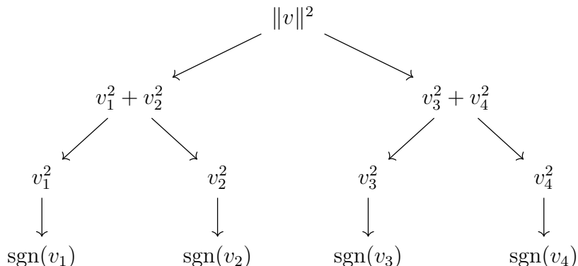
Figure 1: Binary search tree data structure for v \in \mathbb{R}^4 . The leaf nodes store v_i (or equivalently, a weight v_i^2 and the sign of v_i ), and the weight of an interior node is just the sum of the weights of its children. Updates can be done quickly by updating all of the nodes above a particular leaf. Sampling from \mathcal{D}_v can be done by starting from the top of the tree and randomly recursing on a child, with probability proportional to its weight. When v is sparse, the tree can be pruned to only nonzero nodes.
